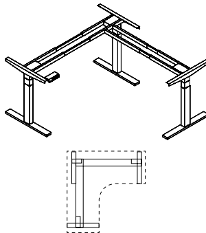
Adjustable Height Electrical L-Unit Base (Sit to stand, fits top sizes below)
