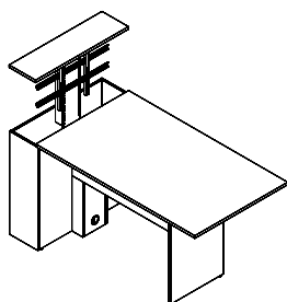
Community Media Table, Box and Trough, Half Panel Leg
