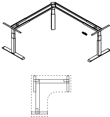
Adjustable Height Electrical L-Unit Base (Sit to stand, fits top sizes below)
